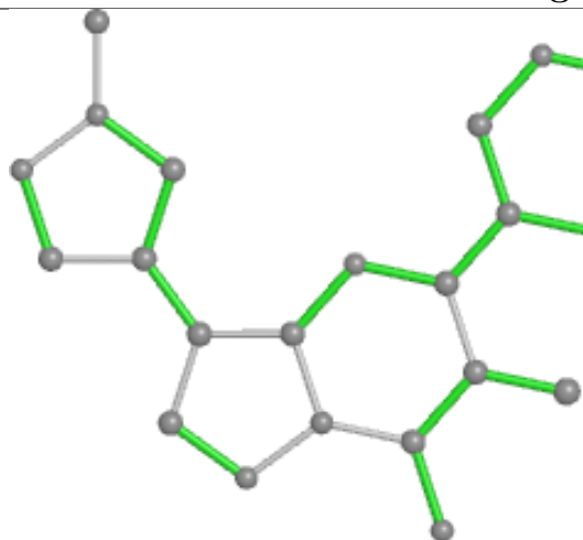
Bond lengths
