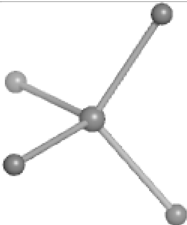
Torsions
