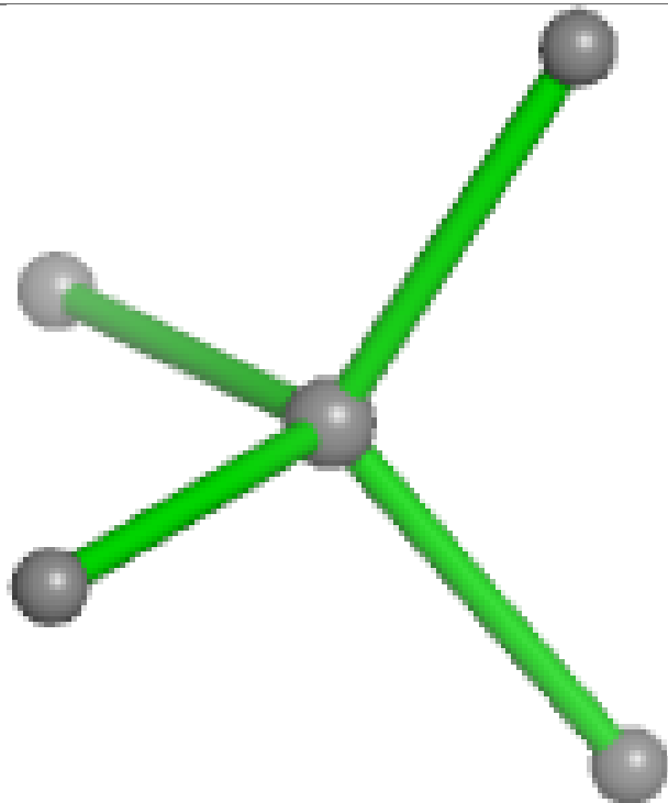
Bond lengths
