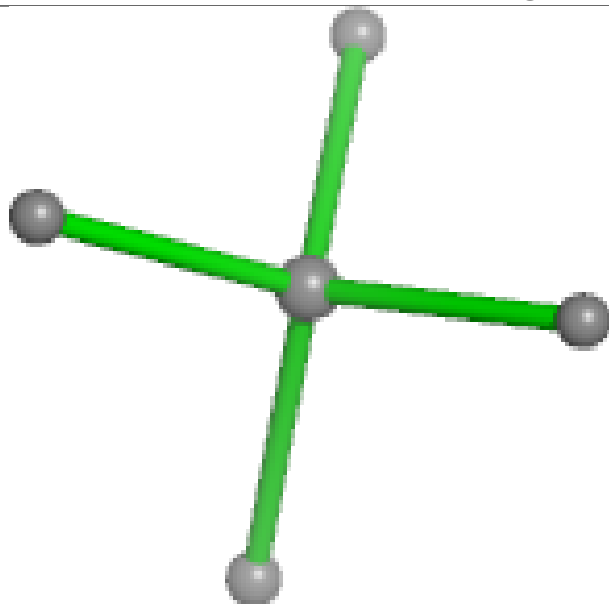
Bond lengths
