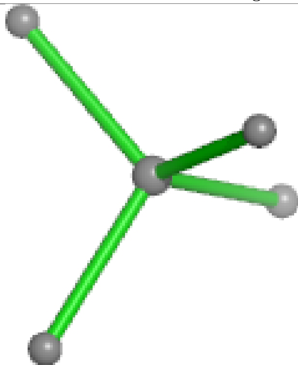
Bond lengths
