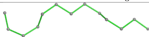
Bond lengths
