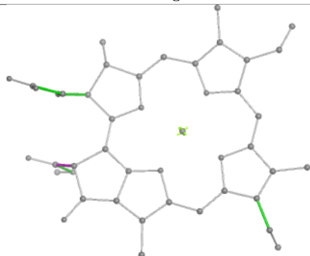
Torsions
