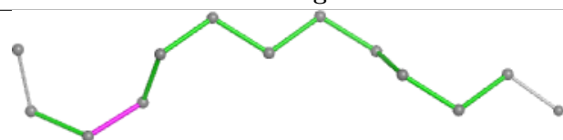
Torsions
