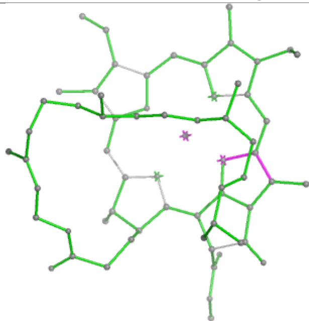
Bond lengths
