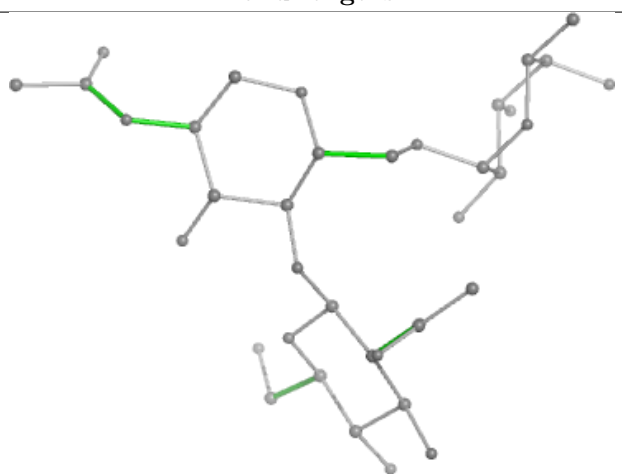
Torsions
