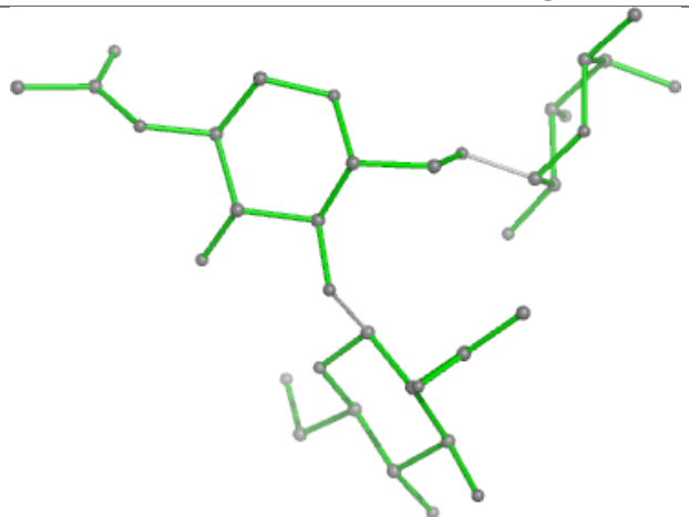
Bond lengths
